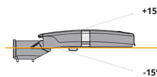
Horizontal assembly
