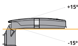
Montage Vertical
