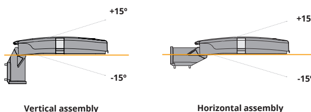
Vertical assembly
