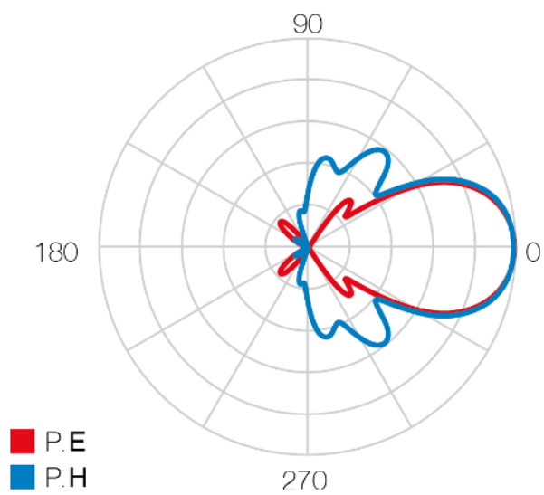
Radiation pattern
