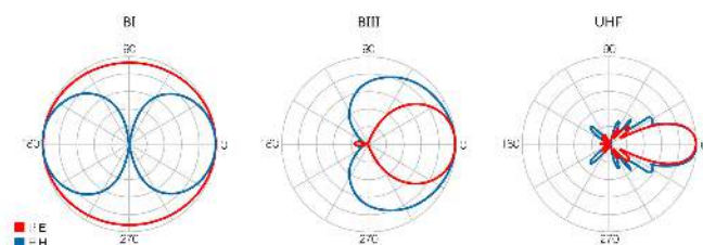
Radiation pattern
