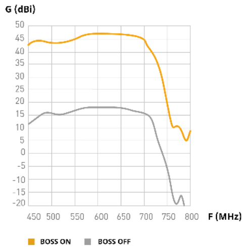
Radiation pattern
