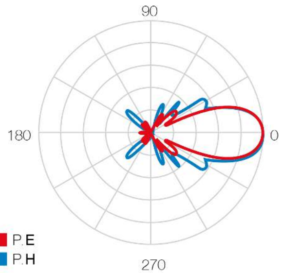
Radiation pattern
