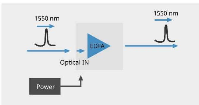
Block diagram
