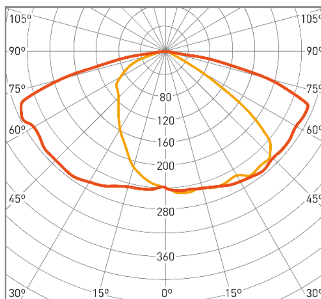
cd/klm ■ C0 - C180 ■ C90 - C270 \eta = 93\% Ljuddistributioner
