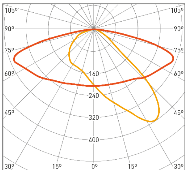
cd/klm ■ C0 - C180 ■ C90 - C270 \eta = 100\% Ljuddistributioner
