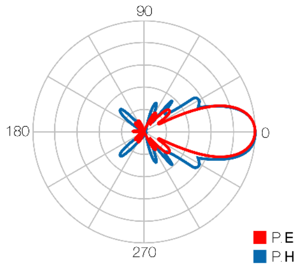
Radiation pattern
